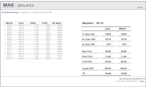
Draft Monitoring
